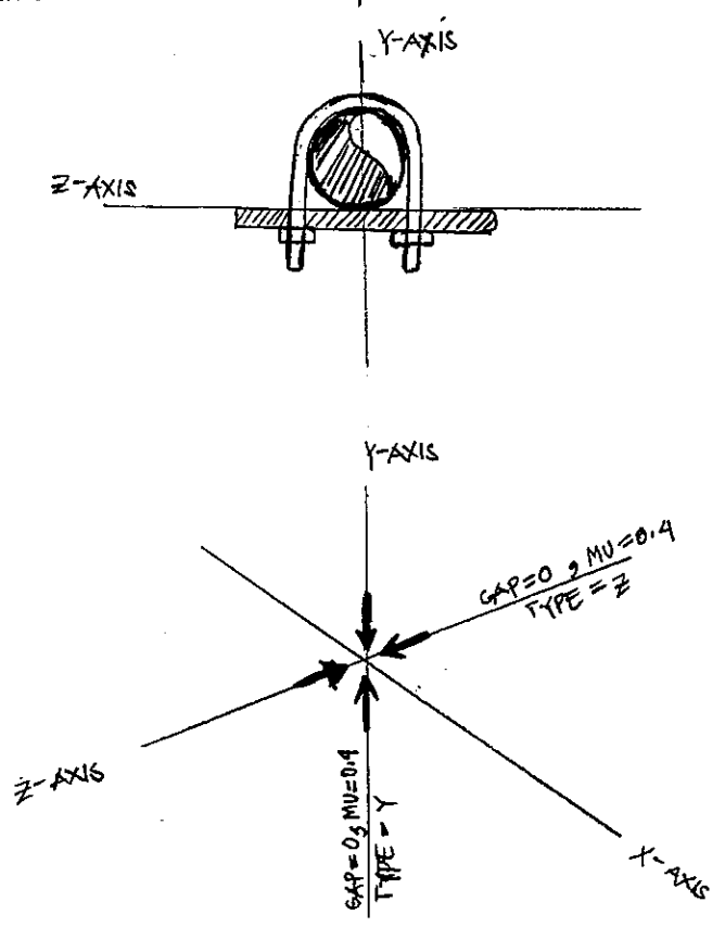
RIGID TYPE U-BOLT
