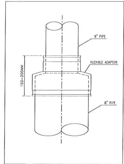
SP-102 TO 107 DETAIL DETAIL-A
