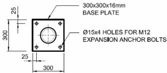
BASE PLATE DETAIL-Y TYP.
